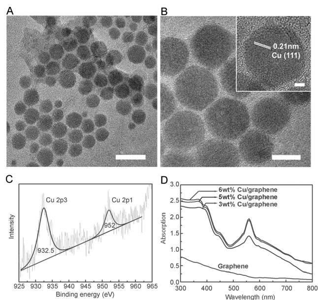
Figure 1. TEM images (A and B; the scale bars are 30 and 10 nm, respectively; the scale bar in the inset of (B) is 2 nm) and XPS profile (C) of 5 wt % Cu/graphene, and UV/Vis absorption spectra of Cu/graphene photocatalysts with different Cu loadings (D).
